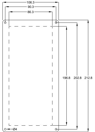
Dimensions in mm's
